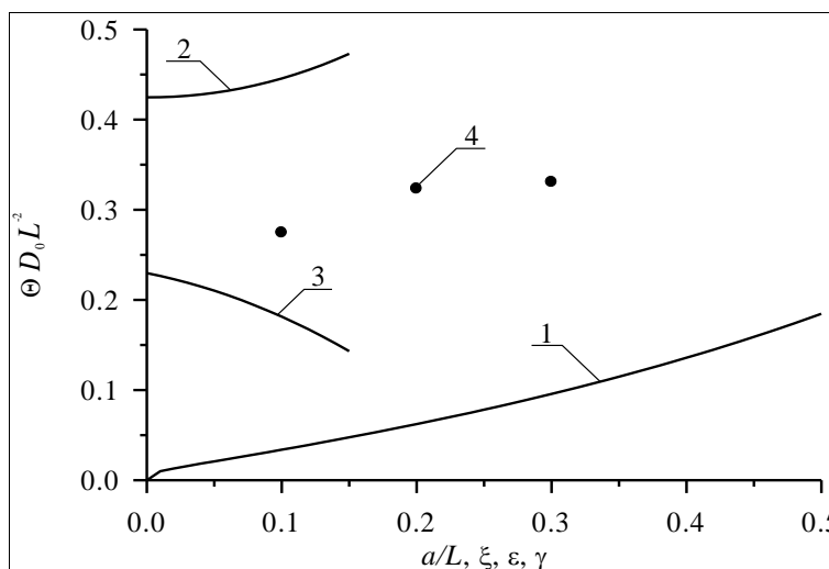
Fig 5a: Dimensionless optimal annealing time of infused dopant as a function of several parameters. Curve 1 describes the dependence of the annealing time on the relation a/L and \xi = \gamma = 0 for equal to each other values of dopant diffusion coefficient in all parts of heterostructure. Curve 2 describes the dependence of the annealing time on value of parameter \epsilon for a/L=1/2 and \xi = \gamma = 0 . Curve 3 describes the dependence of the annealing time on value of parameter \xi for a/L=1/2 and \epsilon = \gamma = 0 . Curve 4 describes the dependence of the annealing time on value of parameter \gamma for a/L=1/2 and \epsilon = \xi = 0
