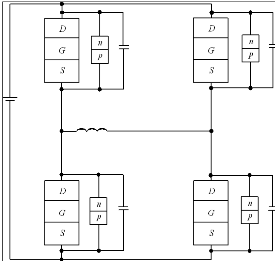
Fig 1a: Structure of the considered converter [15]
