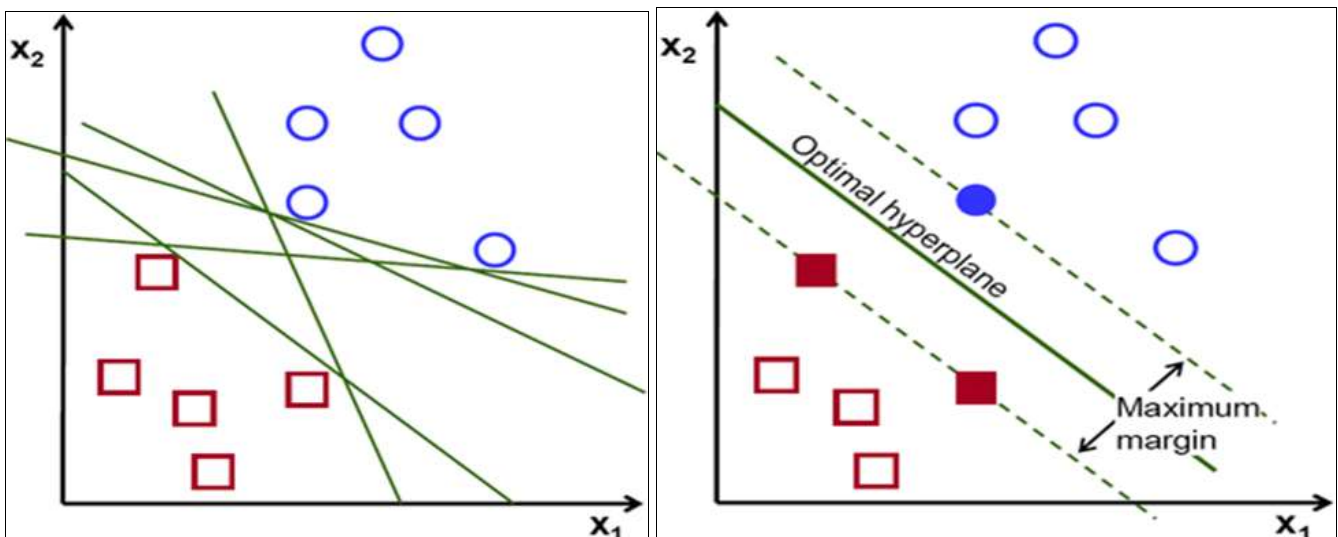
Fig 4: This is a brief overview of how SVM works
